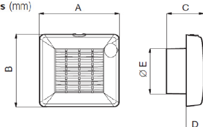
Dimensions (mm)
